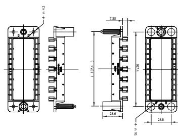
Plastic Docking Frame (for Drawer)
