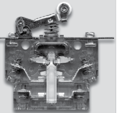
S850 O6A2 f Roller lever, slotted mounting brackets and screw terminal
