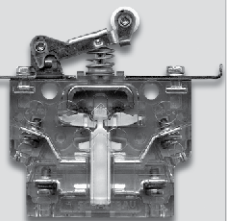
S850 O6A2 d Roller lever, slotted mounting brackets, one of them angled, and screw terminals
