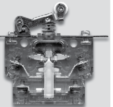
S850 O6A2 b Roller lever, mounting brackets and screw terminals
