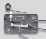
S840 r 20 Roller lever and flat tabs 6.3 x 0.8
