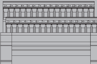
Field terminals view 1371580000 / 1371590000 (AAV141, AAV142, AAV144, AAI543, AAV542, AAV544)
