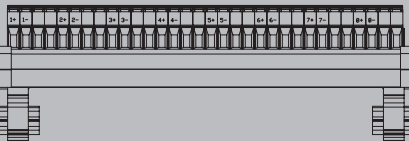
Field terminals view for SAI533
