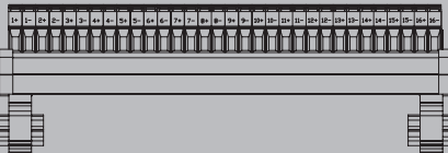
Field terminals view for SAV144
