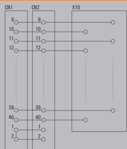
Schematic for 1371470000/1371500000
