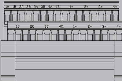
Connection for AAI835
