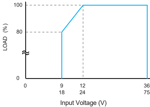
Fig.1 Input voltage derating curve
