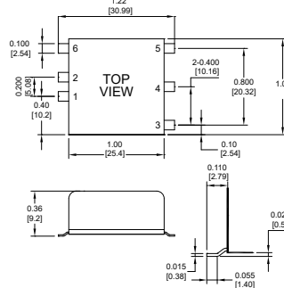
SMD- PACKAGE
