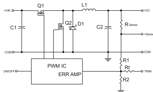
Figure 1.Simplified Schematic
