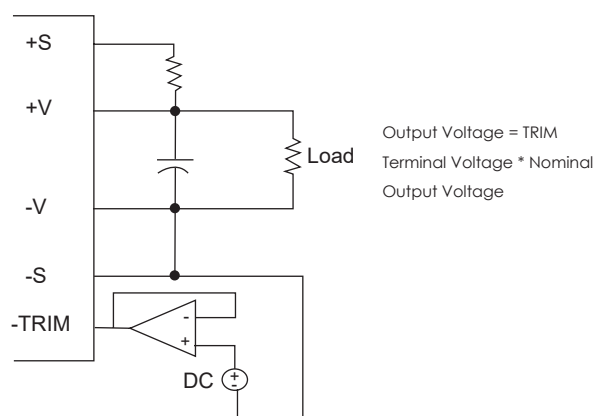
Fig.2 The schematic of output voltage adjusted by using external DC voltage.
