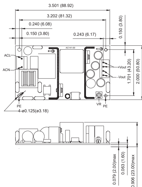
CFM20XXS Series
