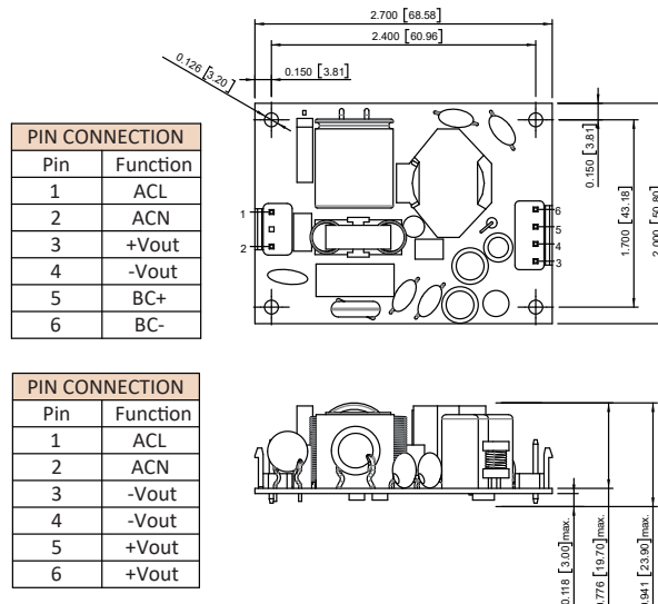
CFM41SXXX-T
