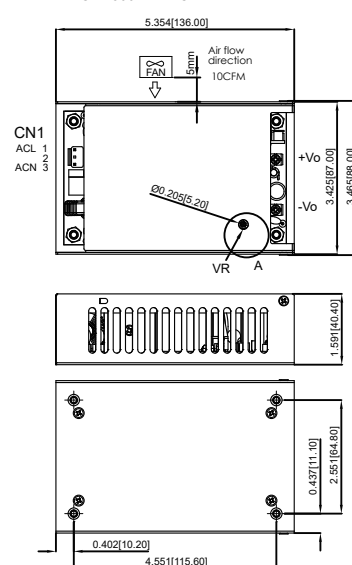
CFM300SXXX-C
