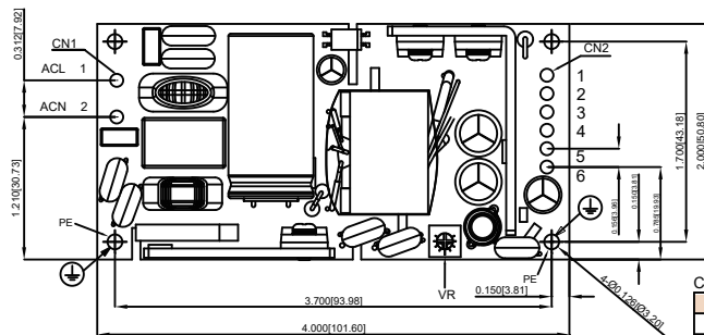
CFM80SXXX-P (Input/Output Connector with PIN)
