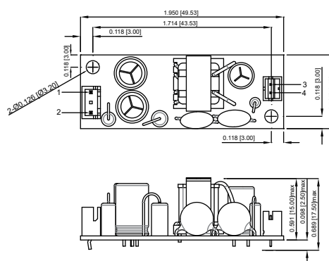
CFM06SXXX-T
