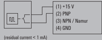
Push pull output cascade
