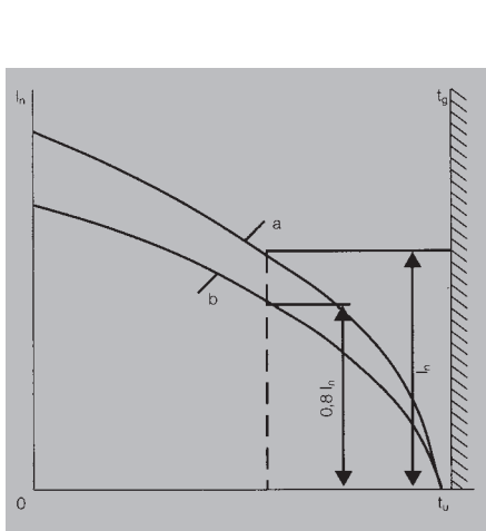
Derating curve
