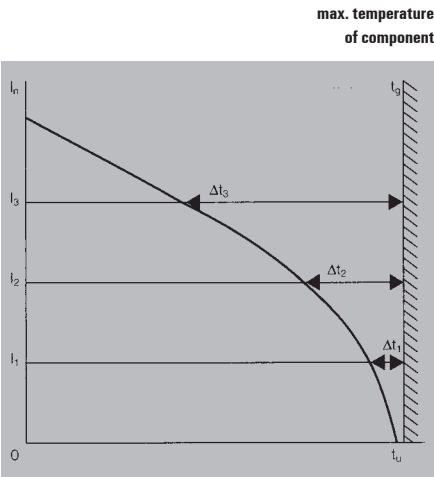
Base curve
