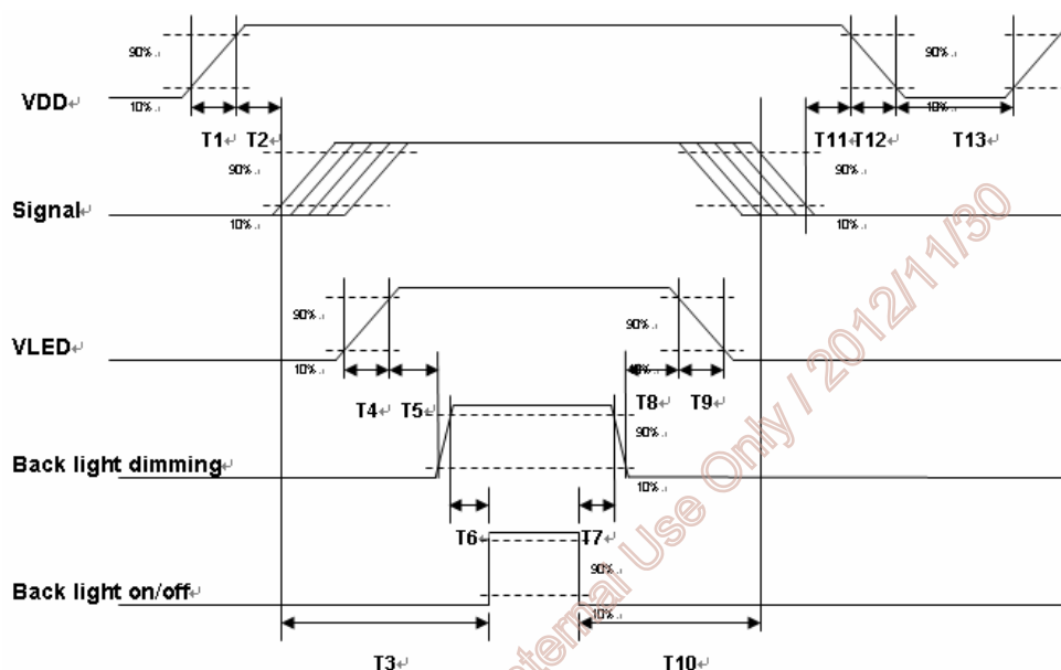
Power ON/OFF sequence timing
